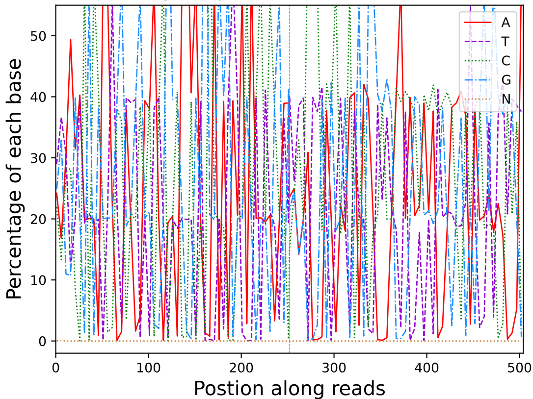
Base percentage along reads (R10503)
